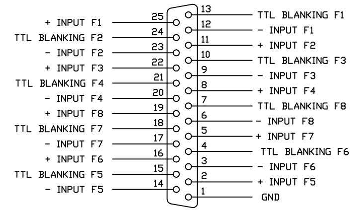
DETAIL A PIN ASSIGNMENTS
